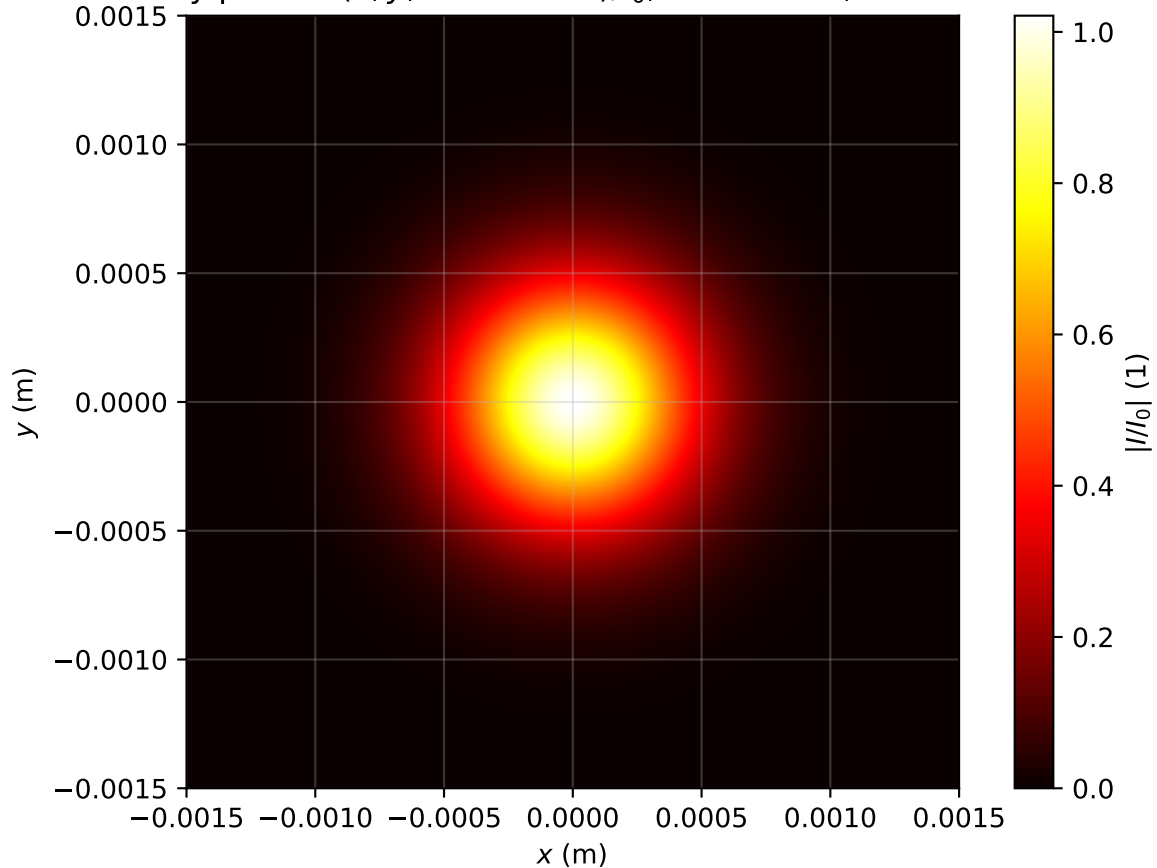
Intensity profile I(x, y, z = 0.637m)/I_0 , Pin=0.4Pcr, artificial time
